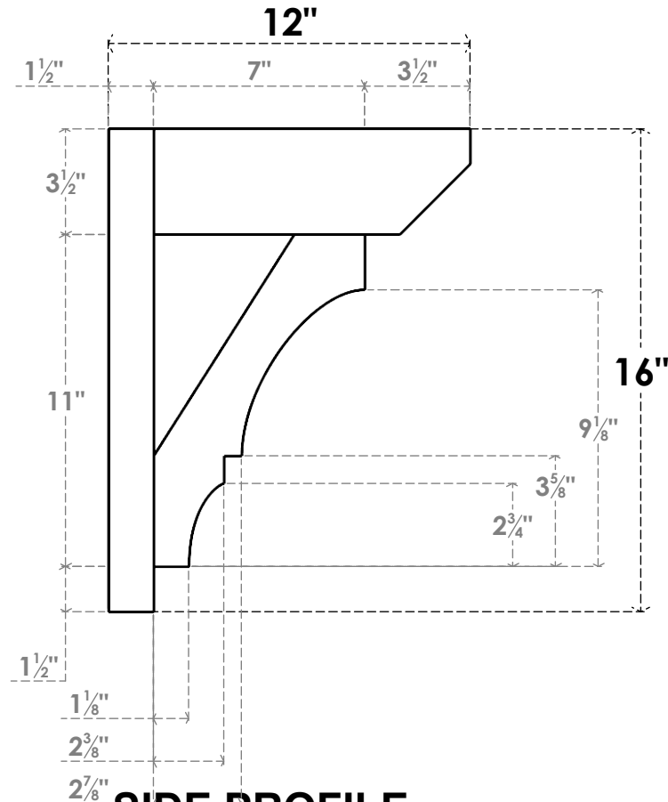
SIDE PROFILE
